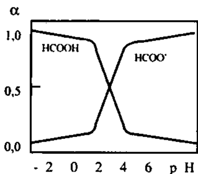
4.1-chizma. Chumoli kislotaning taqsimlanish diagrammasi
