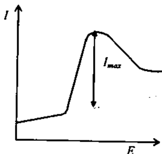
23.14-chizma Ossillopolyarogramma
