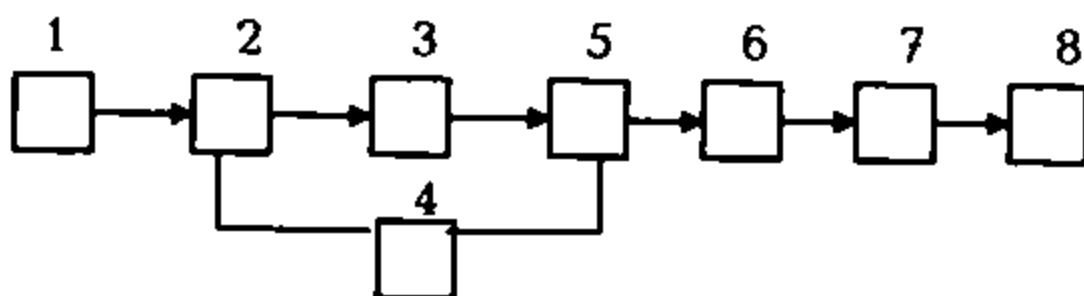
28.3-chizma. Mass-spektrometrning tuzilish sxemasi:
