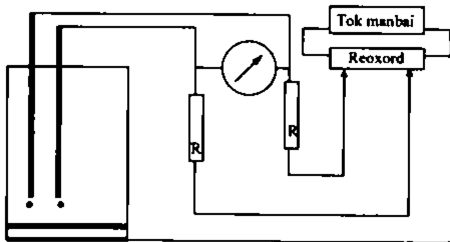
23.11-chizma. Ikkita tomchilaydigan elektrodli differensial polyarografning tuzilishi
