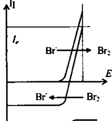
22.13-chizma. Br_2/Br^- jufti voltamper egri chizig'ining fenolni titrlash jarayonida o'zgarishi
