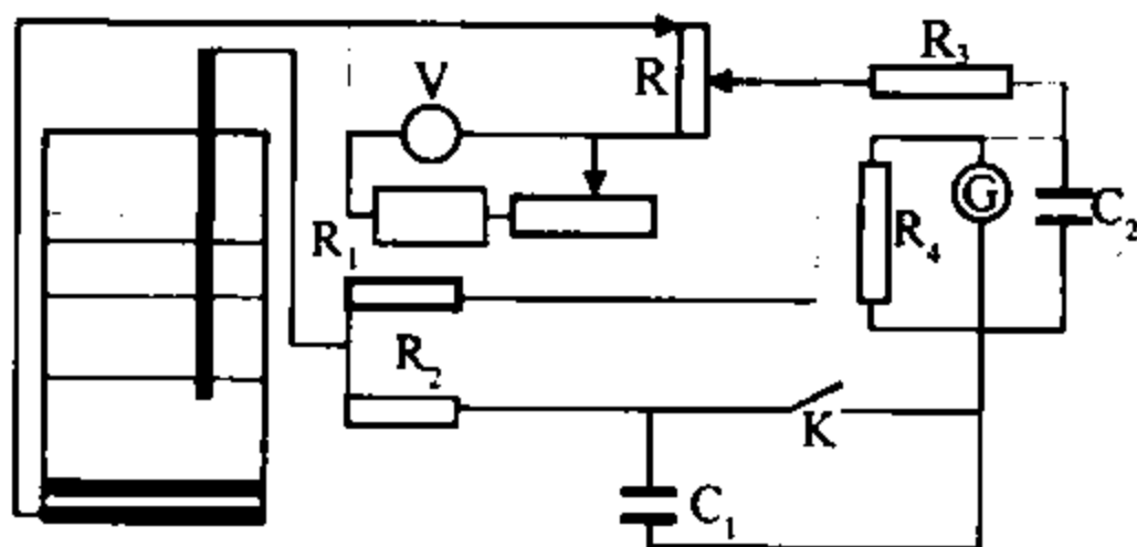
23.12-chizma. Bitta tomchilaydigan elektrodli differensial polyarografning tuzilishi
