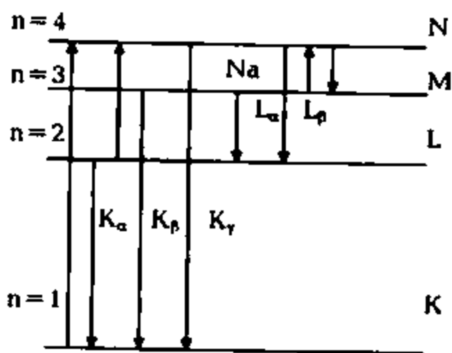
26.7-chizma. Xos rentgen nurlanishining hosil bo'lishi
