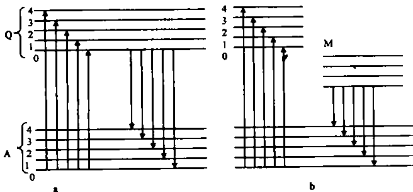
27.7-chizma. Lyuminessent shu'lalanish yuzaga kelishining soddalashtirilgan sxemasi
