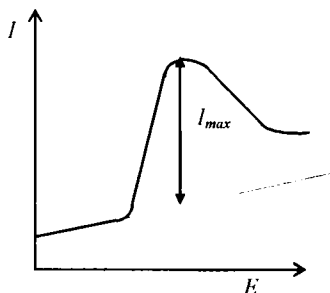
23.14-chizma Ossillopolyarogramma
