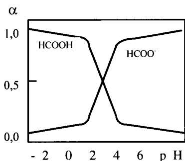
4.1-chizma. Chumoli kislotaning taqsimlanish diagrammasi
