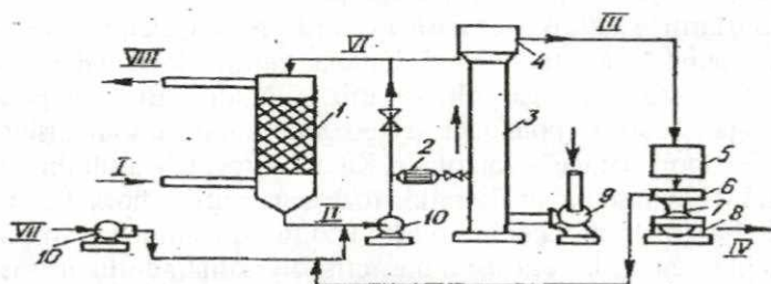
1-rasm. Gazlarni vodorod sulfiddan absorpsion (mishyak sodali) tozalash sxemasi:
