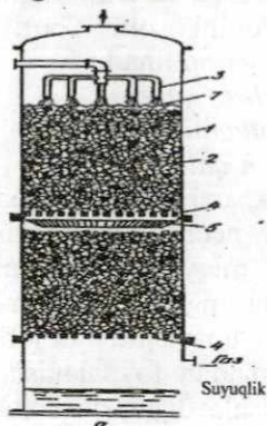
1d-rasm. Nasadkali absorber: 1-silindrsimon qobiq, 2-hasadka, 3-suyuqlikni sohib beruvchi taqsimlagich, 4-nasadka quyiladigan to'r, 5-suyuqlik taqsimlagich, 6-gidravlik zatvor, 7-setka(to'r).
