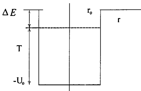
2.1-rasm. Deytron uchun to'g'ri burchakli potentsial o'ra.
