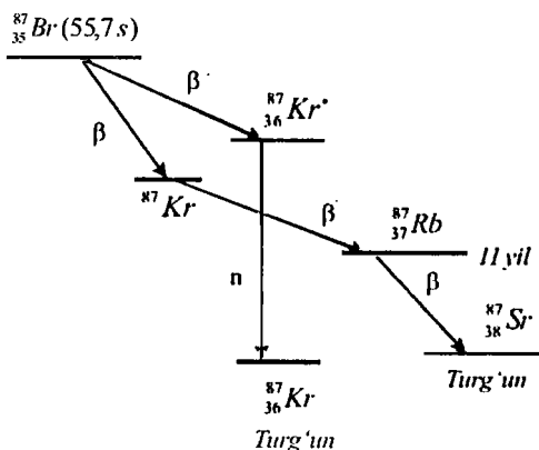
5.14-rasm. Brom-87, Krypton-87, Rubidiy-87 yadrolarining yemirilish sxemalari.
